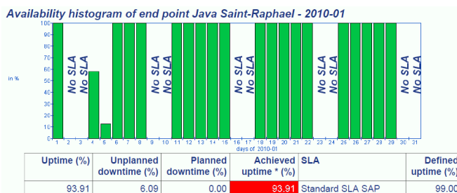
End-to-End Availability Data in SLR for a Java SAP System
